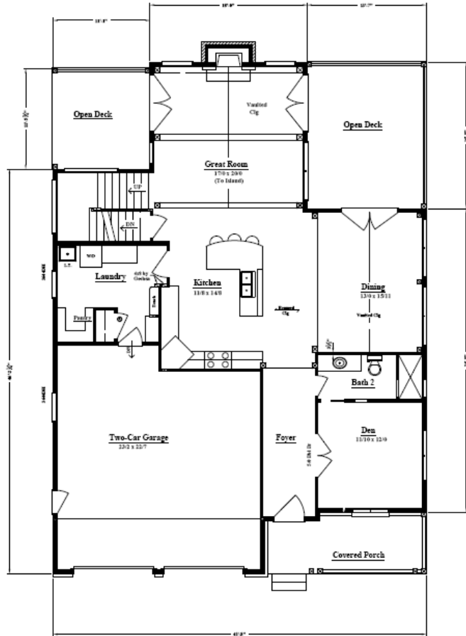
First Floor Plan 1,428 of Living Area
