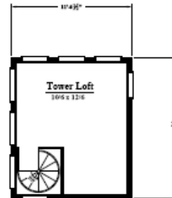
Tower Floor Plan 152 of Living Area
