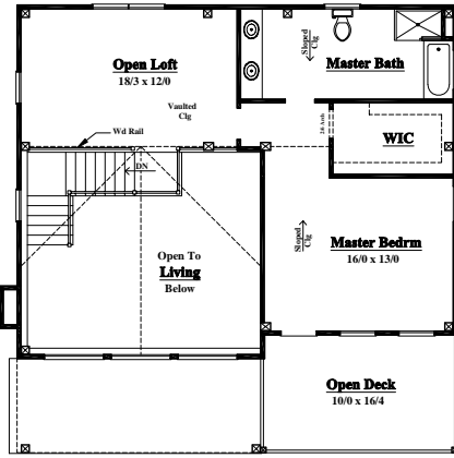
Second Floor Plan 721 sf Living Area
