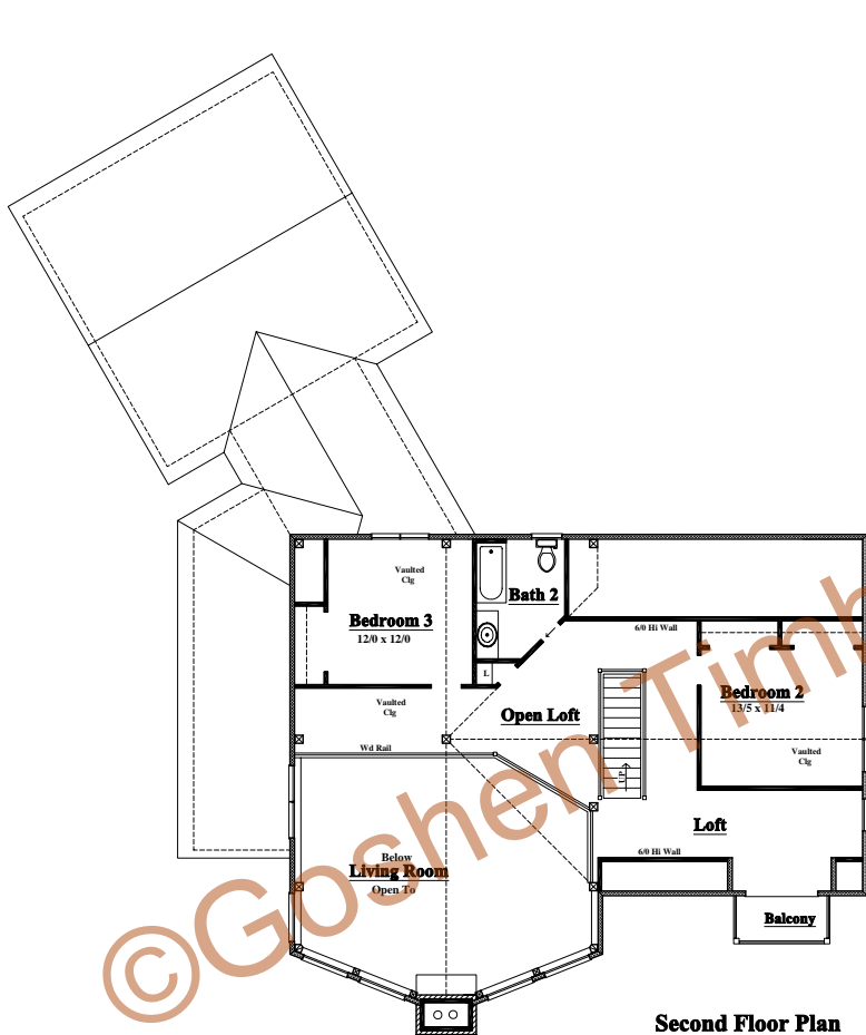
Second Floor Plan 944 sf Living Area
