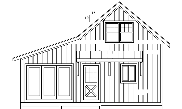
Rear Elevation
