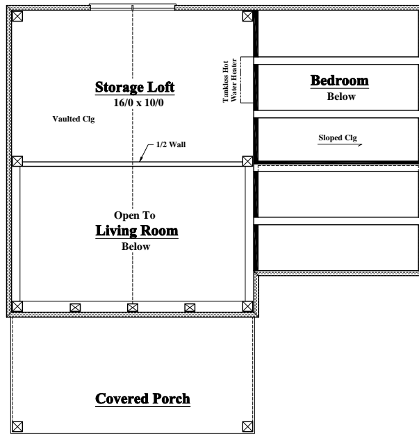
Storage Loft
